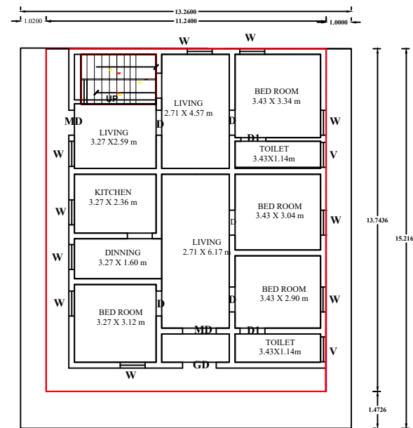
EXIS GROUND FLOOR PLAN
