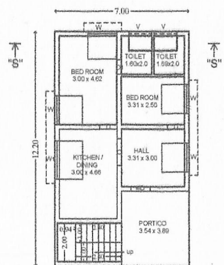
GROUND FLOOR PLAN [ EAST FACING ]
