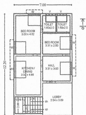
FIRST FLOOR PLAN [ EAST FACING ]
