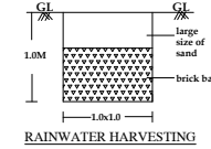
RAINWATER HARVESTING
