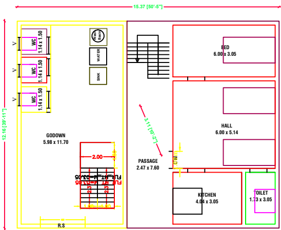
GROUND FLOOR PLAN [NORTH FACING]
