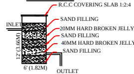
Waste Water Recycle Unit Not To Scale
