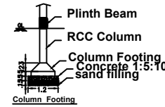
Foundation Detail
