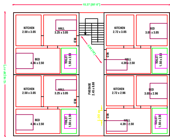
FIRST FLOOR PLAN [NORTH FACING]
