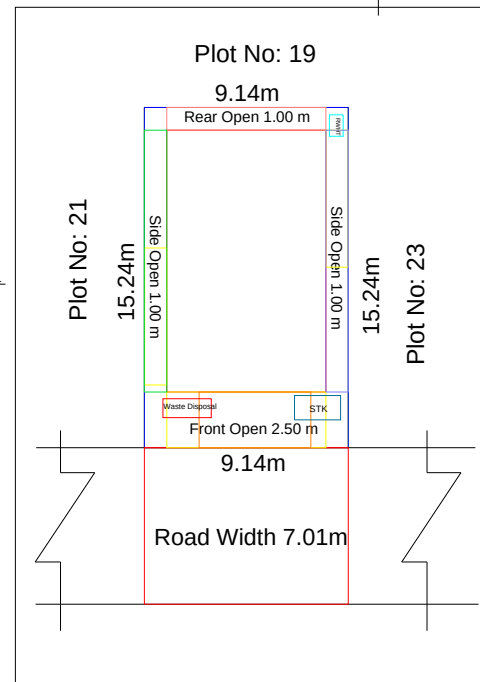
Site Plan
