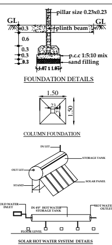
SOLAR HOT WATER SYSTEM DETAILS
