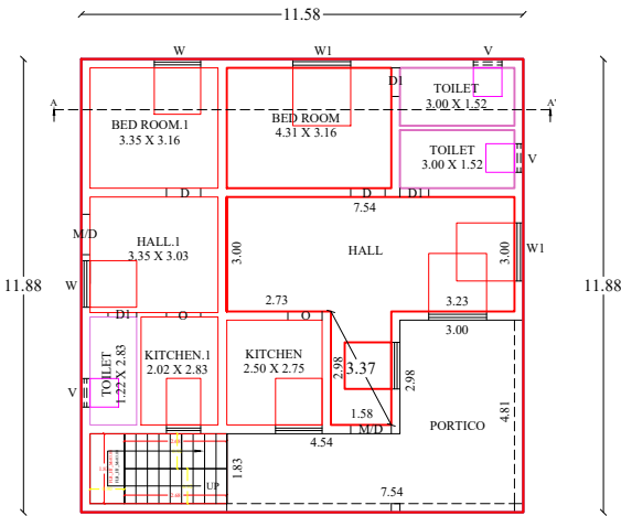
GROUND FLOOR PLAN (EAST FACING)
