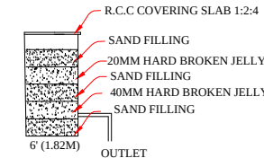
Waste Water Recycle Unit Not To Scale
