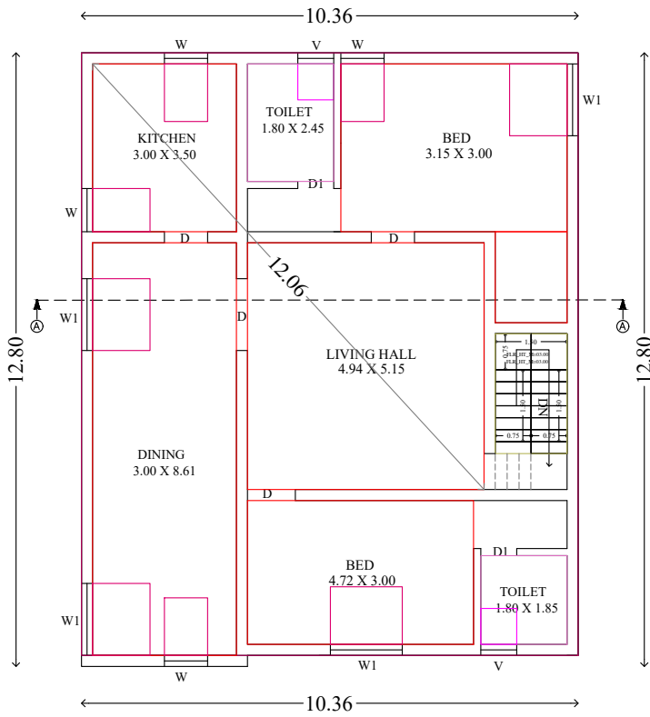
PROPOSED FIRST FLOOR (NORTH FACING)
