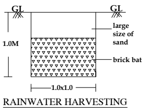
RAINWATER HARVESTING
