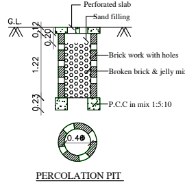
PERCOLATION PIT
