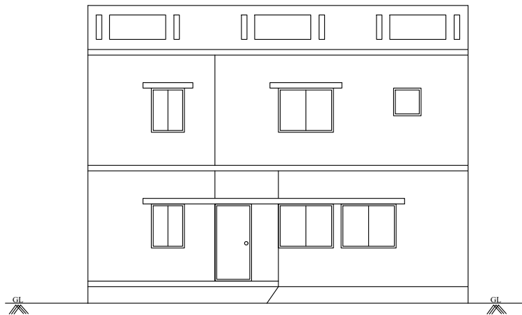
FRONT ELEVATION
