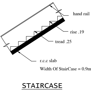
STAIRCASE
