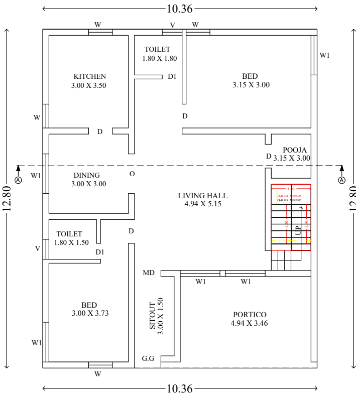
EXISTING GROUND FLOOR (NORTH FACING)
