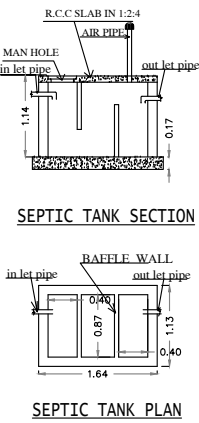
SEPTIC TANK PLAN
