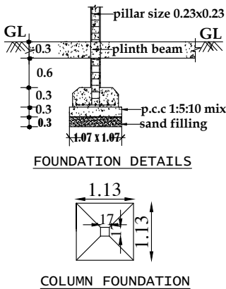
COLUMN FOUNDATION
