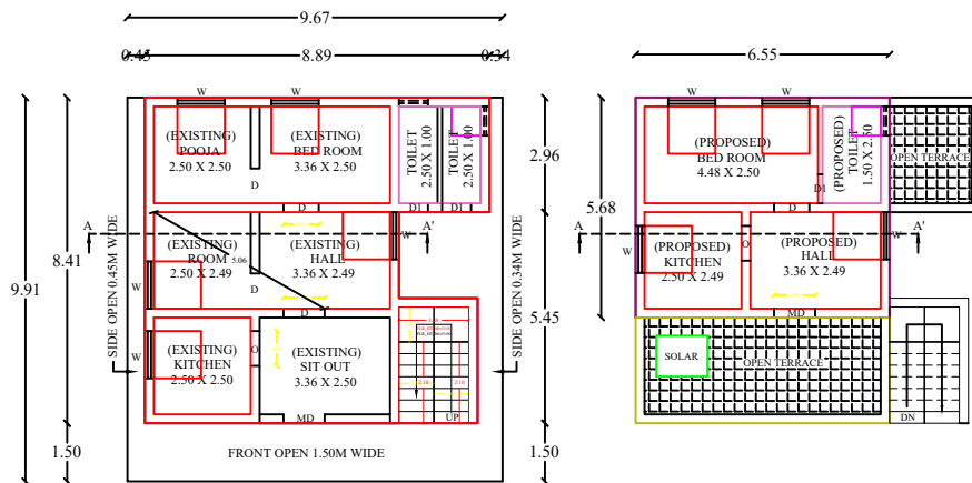
FIRST FLOOR PLAN (PROPOSED BUILDING)
