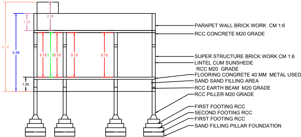
SECTIONAL VIEW
