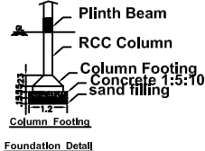
Foundation Detail
