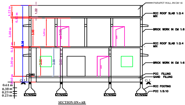
SECTION ON-AB
