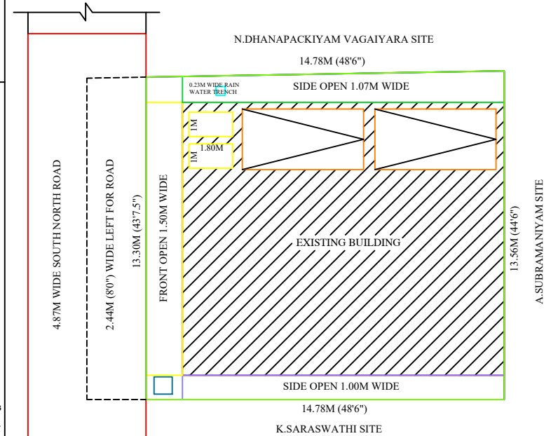
SITE PLAN
