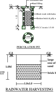
RAINWATER HARVESTING
