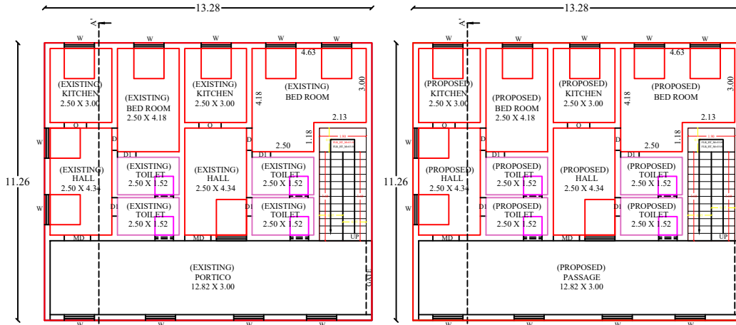
GROUND FLOOR PLAN (EXISTING BUILDING) (NORTH FACING)
