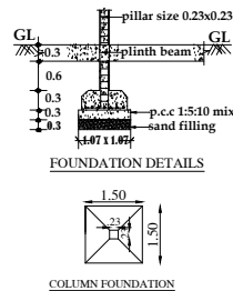
COLUMN FOUNDATION
