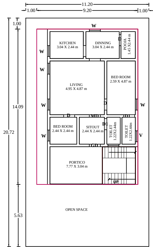
EXIS GROUND FLOOR PLAN
