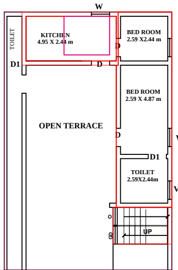
EX & PRO FIRST FLOOR PLAN
