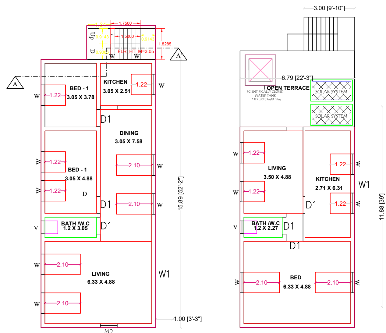
GROUND FLOOR PLAN - WEST FACING
