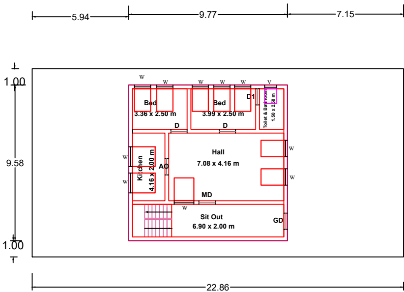
Ground Floor Plan ( East Facin)
