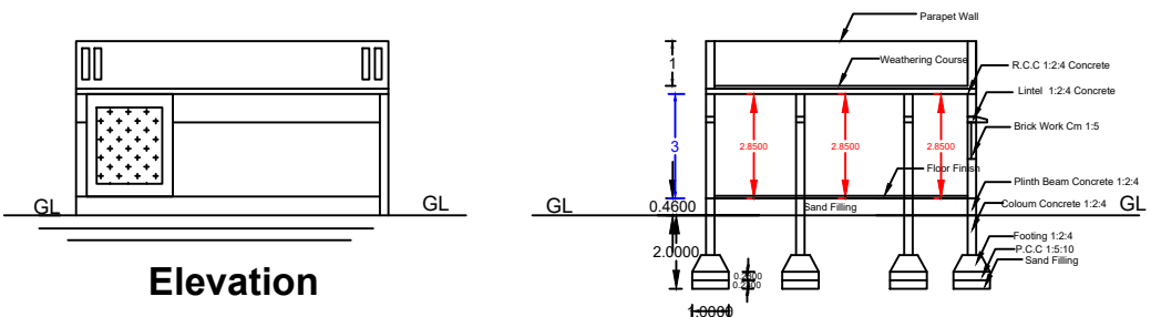
Section Section - AA
