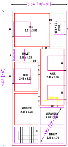
PRO. GROUND FLOOR PLAN [ EAST FACING ]
