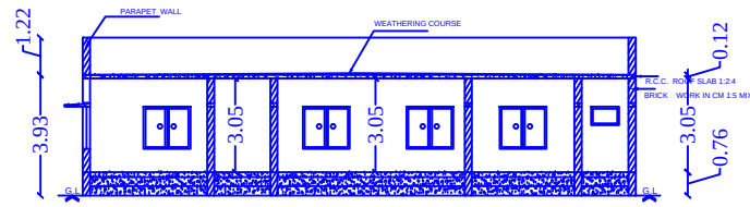
Section on-"AA"
