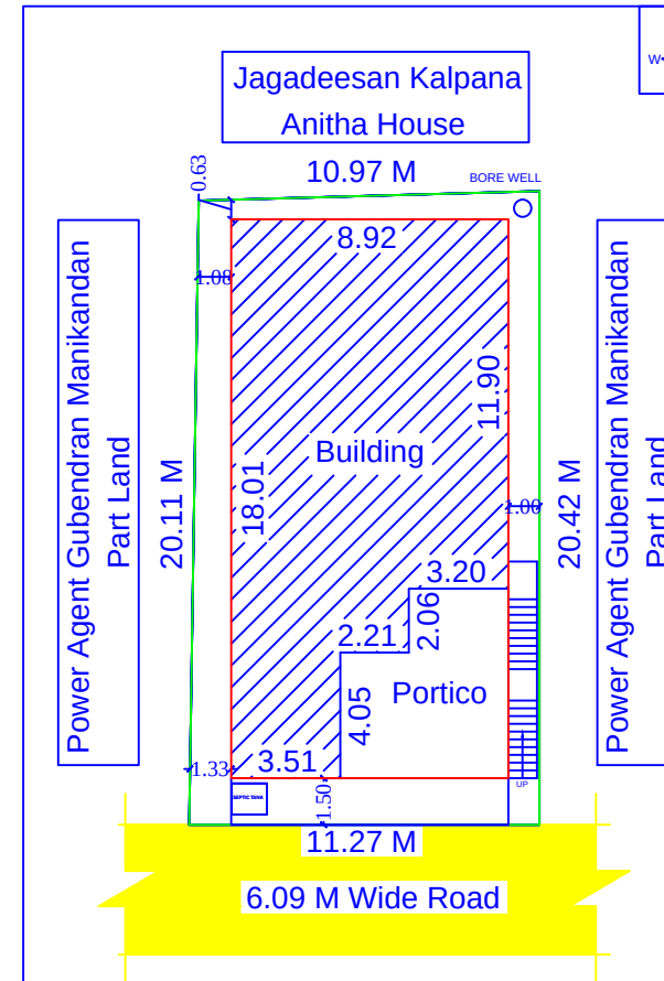
SITE PLAN
