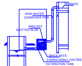
RAIN WATER HARVESTING SYSTEM
