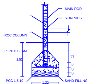
COLUMN DETAILS
