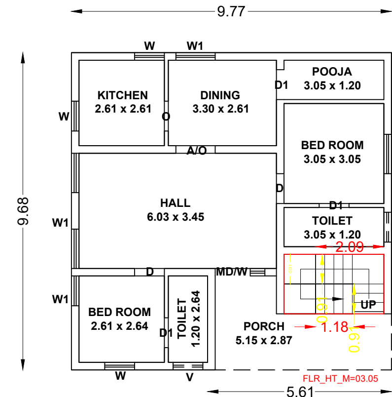
EXISTING GROUND FLOOR PLAN (NORTH FACING)
