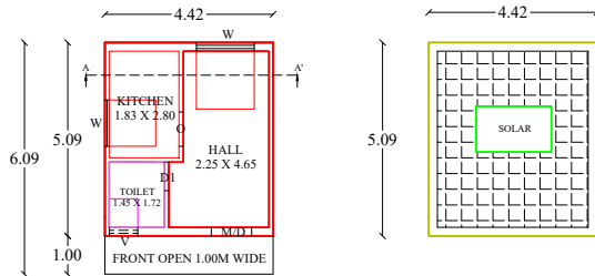
GROUND FLOOR PLAN (EAST FACING)
