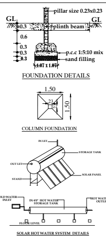
SOLAR HOT WATER SYSTEM DETAILS
