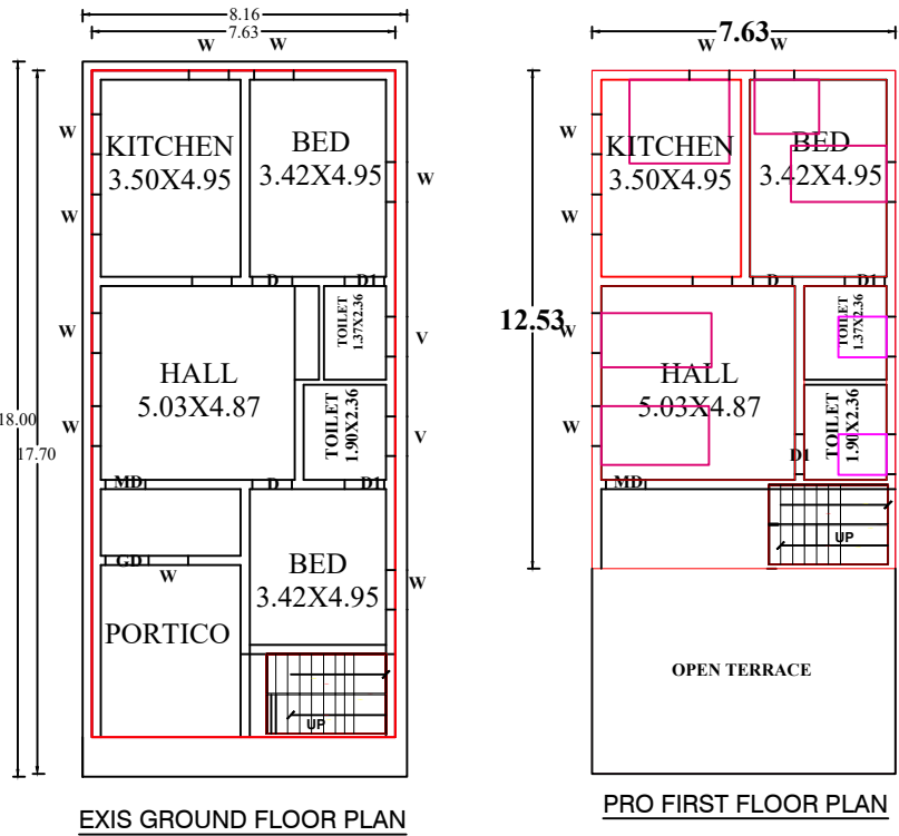
EXIS GROUND FLOOR PLAN
