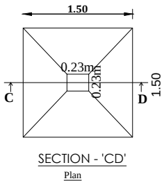
SECTION - 'CD'
