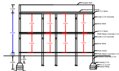
SECTION SECTION - AB
