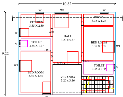
GROUND FLOOR PLAN (NORTH FACING)
