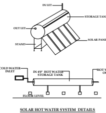
SOLAR HOT WATER SYSTEM DETAILS
