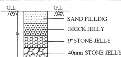
RAIN WATER HARVESTING RECHARGE PIT
