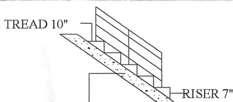
STAIRCASE DETAILS
