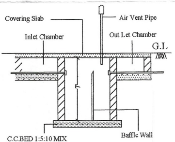
SECTION ON S.Tank
