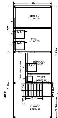
GROUND FLOOR PLAN SCALE 1:100
