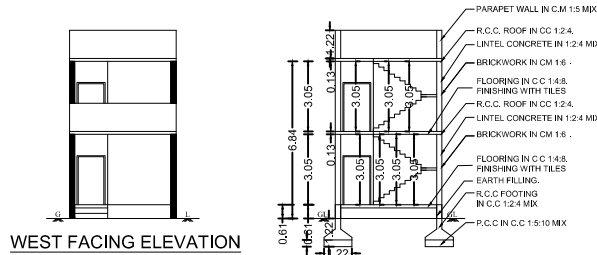
WEST FACING ELEVATION
