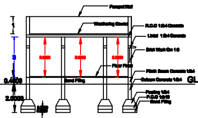
Section Section - AA
