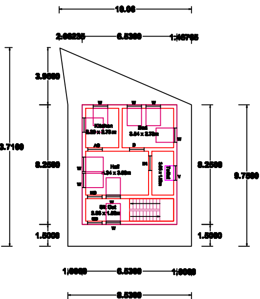
GROUND FLOOR PLAN ( NORTH FACING )
