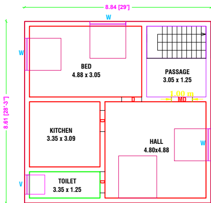
PRO. FIRST FLOOR PLAN [WEST FACING]
