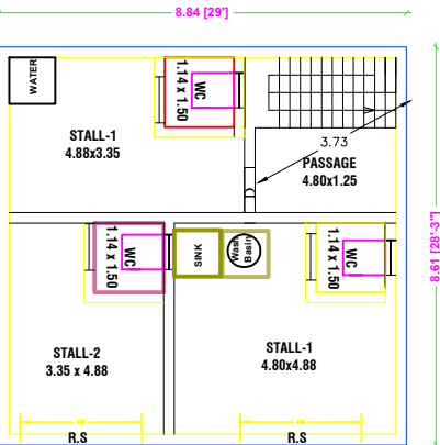
PRO. GROUND FLOOR PLAN [EAST FACING]
