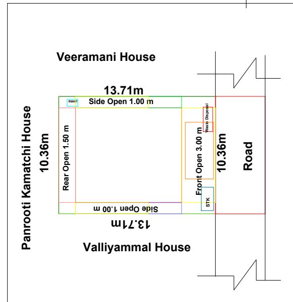
Site Plan
