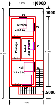
PROPOSED GROUND FLOOR PLAN
