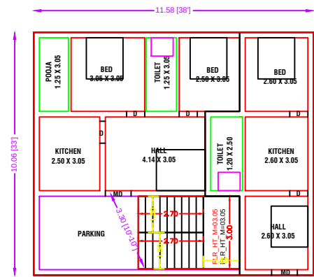
PRO. GROUND FLOOR PLAN [ EAST FACING ]
