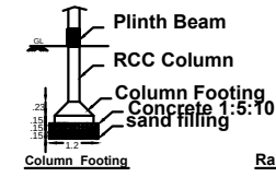
Foundation Detail
