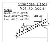
Staircase Detail
