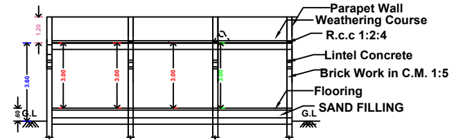
SECTION ON "BB"
