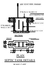
SEPTIC TANK DETAILS SCALE: 1:400
