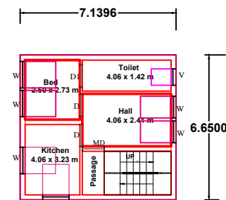
First Floor
