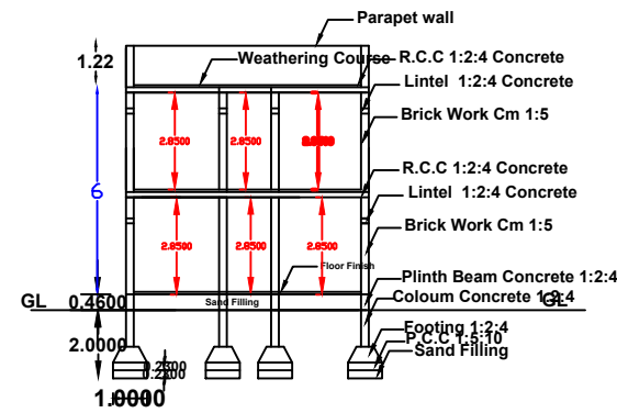
Section Section - AA
