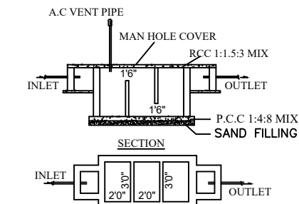
RAIN WATER HARVESTING TANK (Not to scale)
