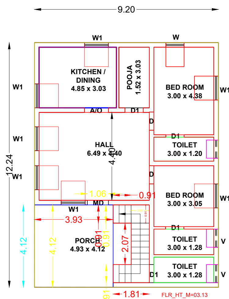
GROUND FLOOR PLAN (NORTH FACING)
