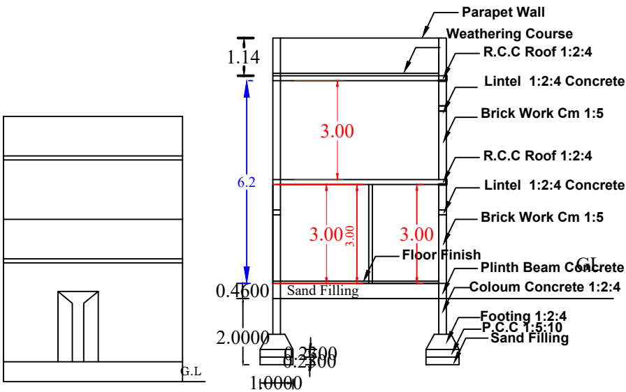
ELEVATION Section - AA
