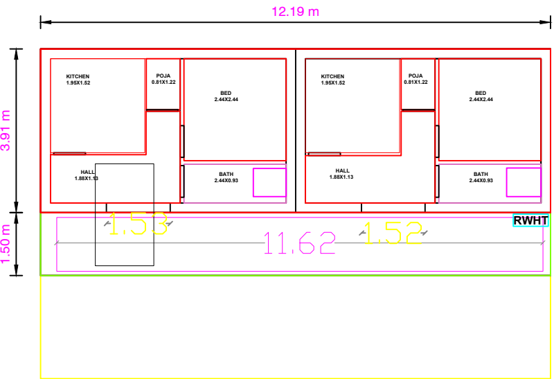
GROUND FLOOR PLAN (FACEING OF EAST)
