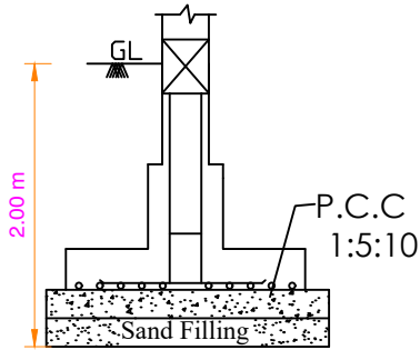
Isolated Footing - A (1.50X1.50) (Not to Scale)
