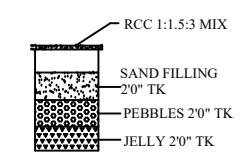
RAIN WATER HARVESTING TANK
