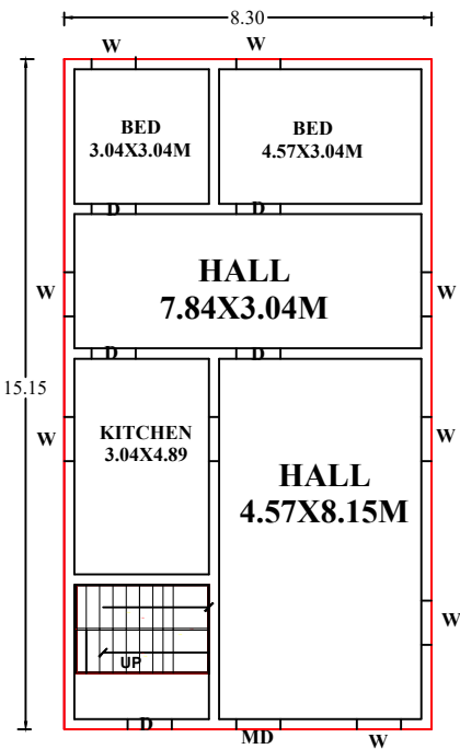
EXIS GROUND FLOOR PLAN
