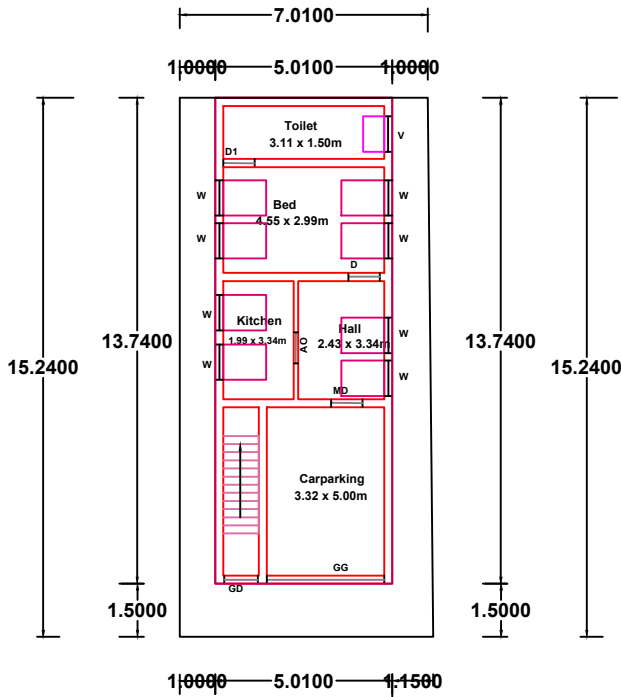
GROUND FLOOR (East Facing)
