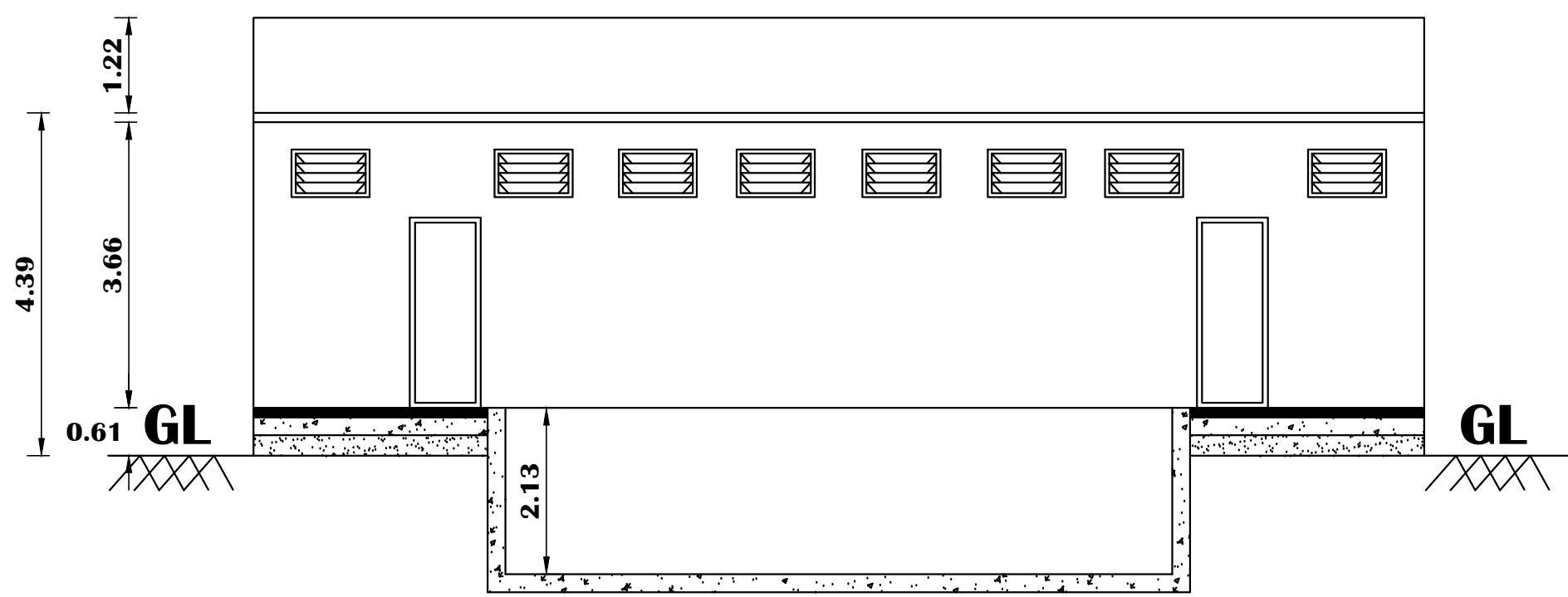
SECTION BB
