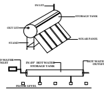
SOLAR HOT WATER SYSTEM DETAILS
