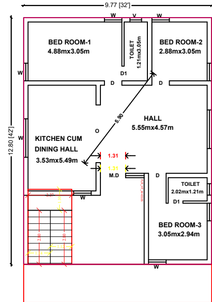
EXT.GROUND FLOOR PLAN
