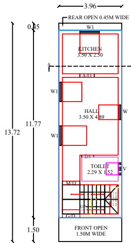
GROUND FLOOR PLAN (NORTH FACING)
