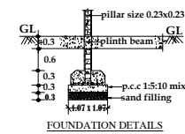
FOUNDATION DETAILS
