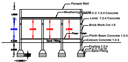
Section Section - AA
