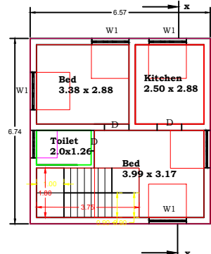
Proposed First Floor Plan (Residential)
