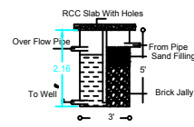
RWHS Tank Details
