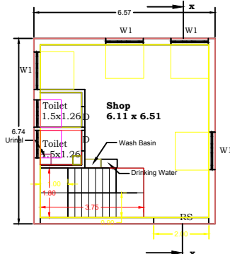
Proposed Ground Floor Plan (Shop)
