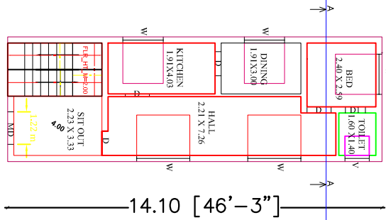
GROUND FLOOR PLAN (EAST FACING)
