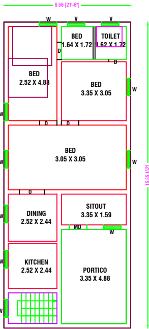
PRO. GROUND FLOOR PLAN [EAST FACING]
